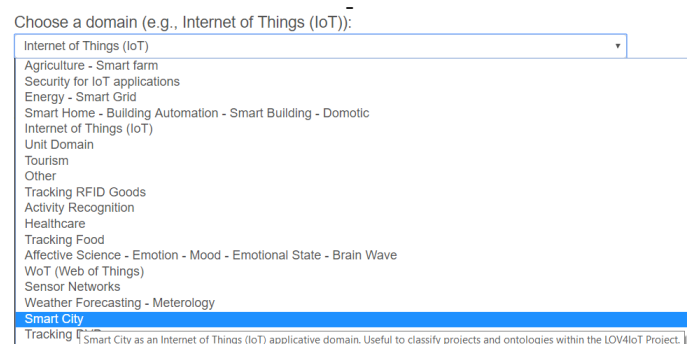
Fig. 2. Drop-down-list displaying the result provided by the web service and the SPARQL result.
