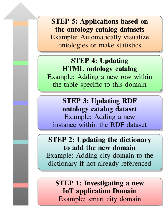
Fig. 1. Overview of the methodology to update ontology catalogs
