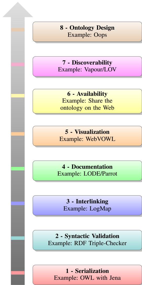
Fig. 3. Ontology quality methodology
