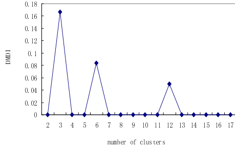
Fig. 17. DMDI curve of lenses at Min-support=0.8
