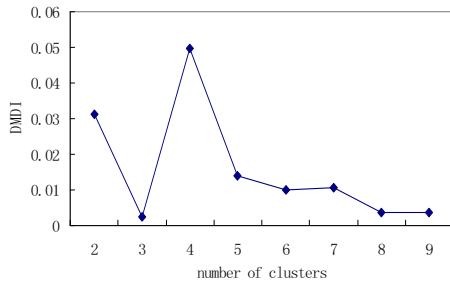
Fig. 19. DMDI curve of soybean-small at Min-support=0.8
